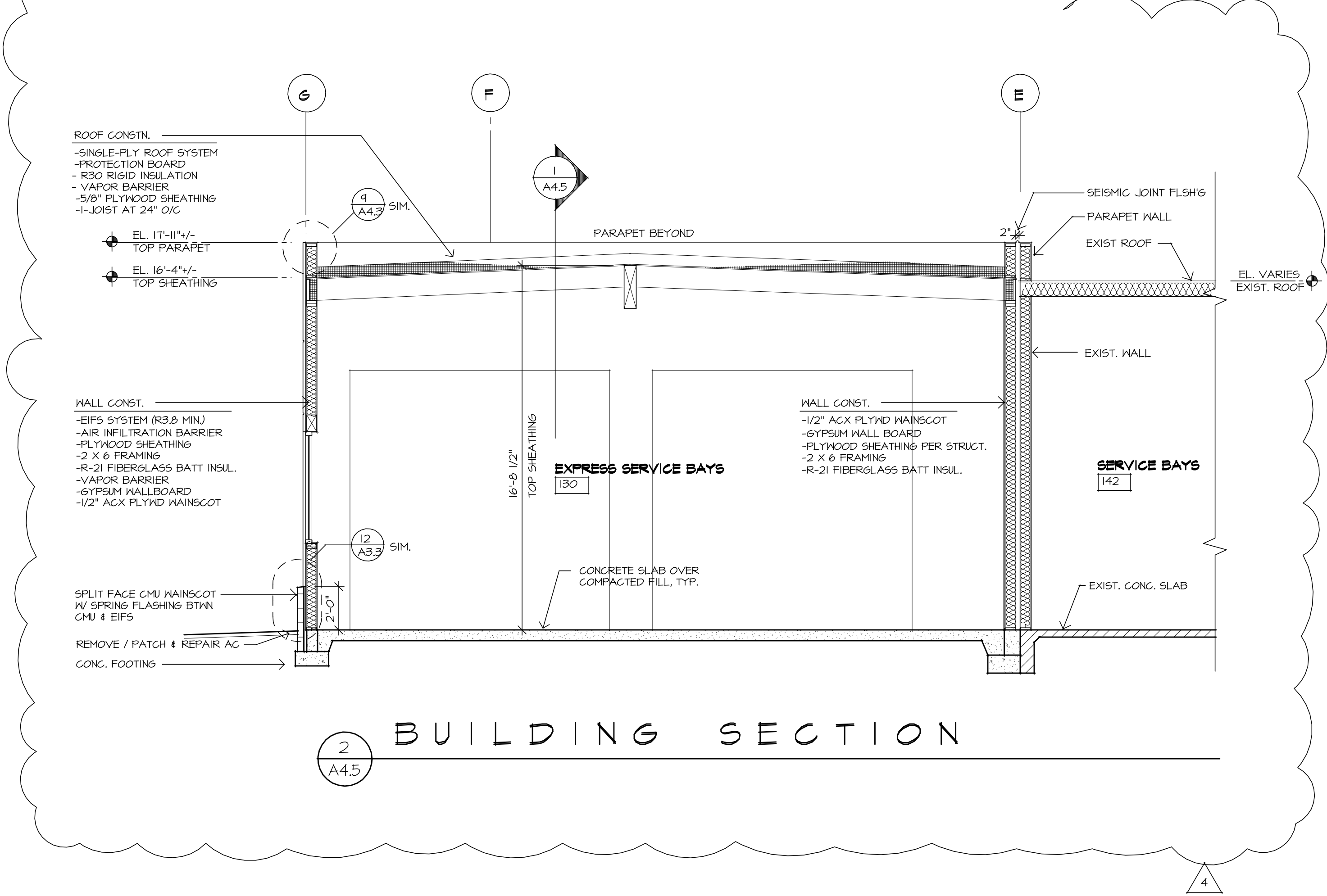
BUILDING SECTION
